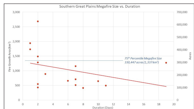
Figure 8. Southern Great Plains megafire size versus duration with linear trend line (red) and 75th percentile fire size denoted (blue).
