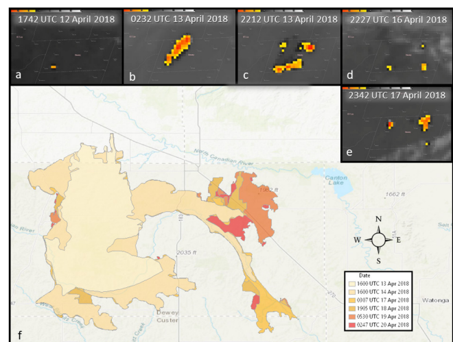
Figure 14. Geostationary Operational Environmental Satellite (GOES)-16 3μm imagery of Rhea Fire evolution between 1742 UTC 12 April 2018 and 2342 UTC 17 April 2018, and f) Rhea Fire progression map.
